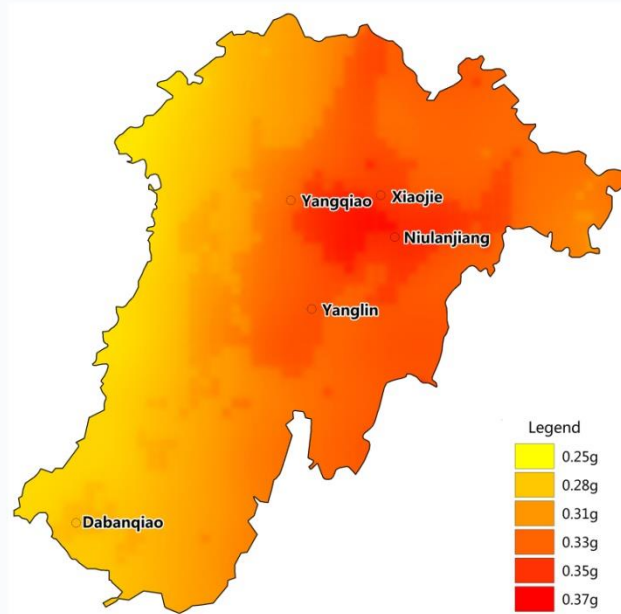
Figure 2: Site Peak Ground Acceleration Map for Songming, Yunnan Province
