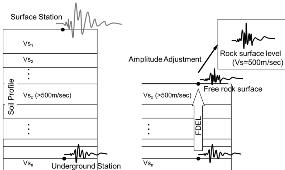
Figure 3 Schematic diagram for calculation of rock surface ground motion with shear wave velocity of 500m/sec
