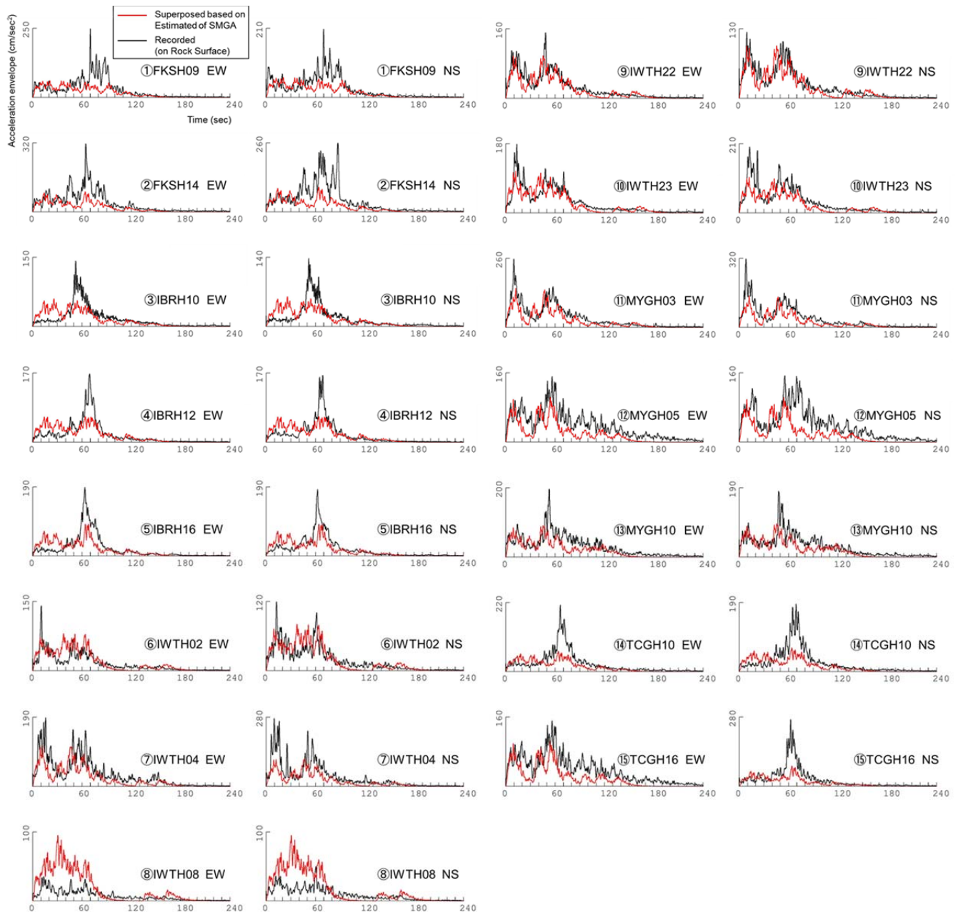
Figure 5 Comparison of Acceleration envelopes of recorded and simulated acceleration time histories
