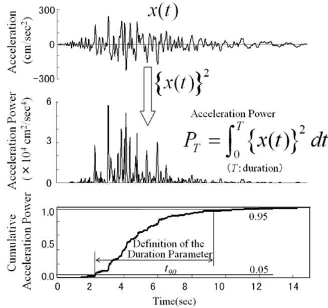
Figure 2 Definition of duration parameter t_{90} with acceleration total power P_T
