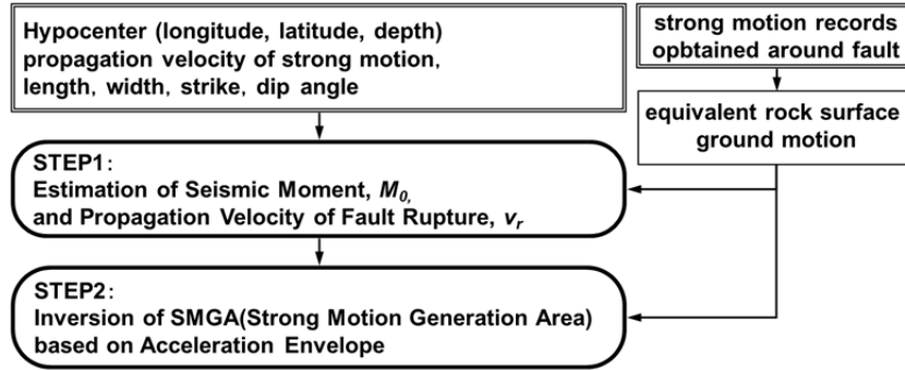
Figure 1 Outline for inversion of source process
