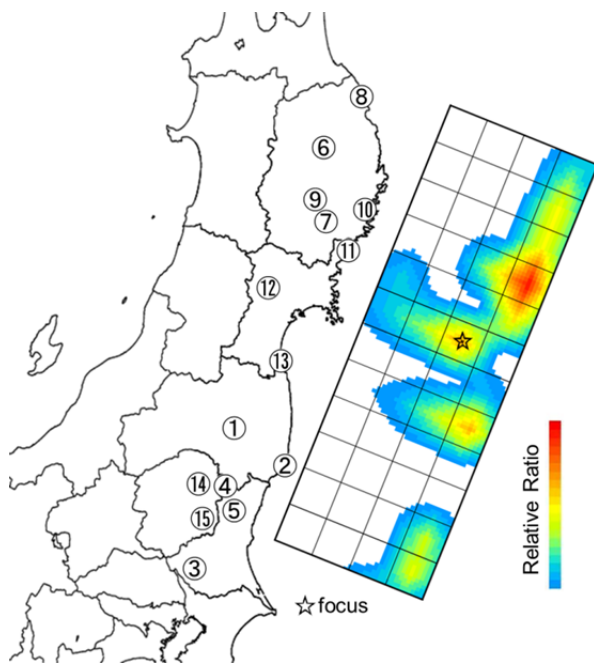
Figure 4 Location of strong motion stations and fault plane (distribution on fault plane is estimated SMGA. The circled number represents location of observation stations.)
