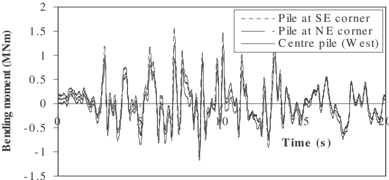
Figure 6. Pile bending moment close to the bottom of the loose sand layer ( z = -9.1 m) observed for 3 piles in the group.
