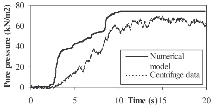
Figure 3. Pore pressure generation at the middle of the loose Nevada sand layer.
