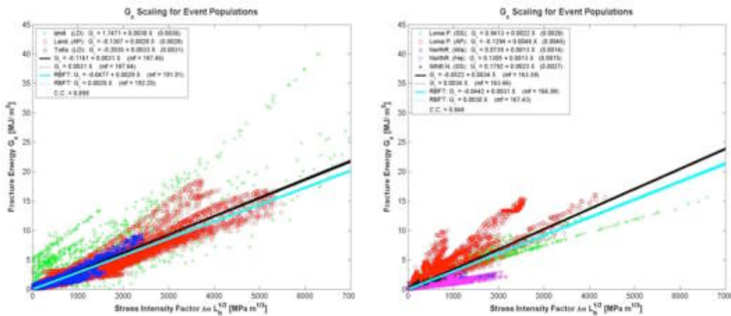
Figure 5. Distribution of fracture energy (vertical axis) and stress intensity factor (horizontal axis) for surface rupture (left) and buried rupture (right) events. Source: Mai et al. (2005).
