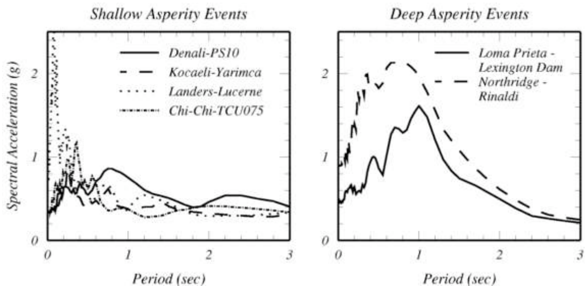
Figure 1. Near-fault response spectra of recent large earthquakes. Left: Four earthquakes, M_w 7.2 to 7.9, with shallow asperities and large surface faulting. Right: Two earthquakes, M_w 6.7 and 7.0, with deep asperities and no surface faulting.
