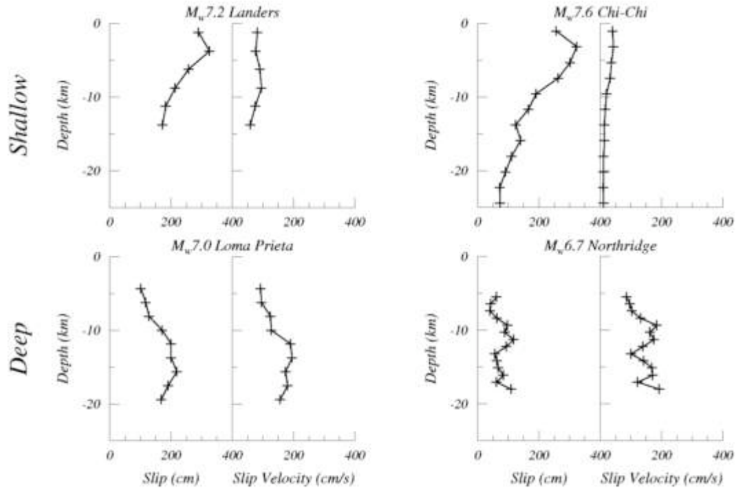
Figure 4. Distribution of slip (left panel) and slip velocity (right panel) for shallow (top) and deep (bottom) earthquakes. The left hand side compares two strike slip earthquakes and the right hand side compares two thrust earthquakes.
