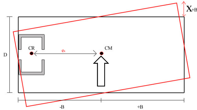
Figure 2. Plan view of building type 2 with two C-shaped walls
