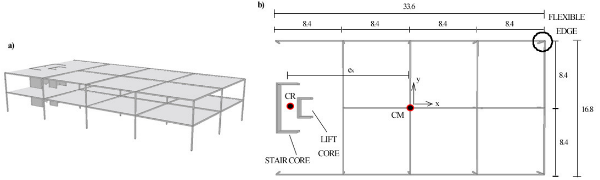
Figure 1. (a) Isometric and (b) plan view of building type 1 with two C-shaped walls
