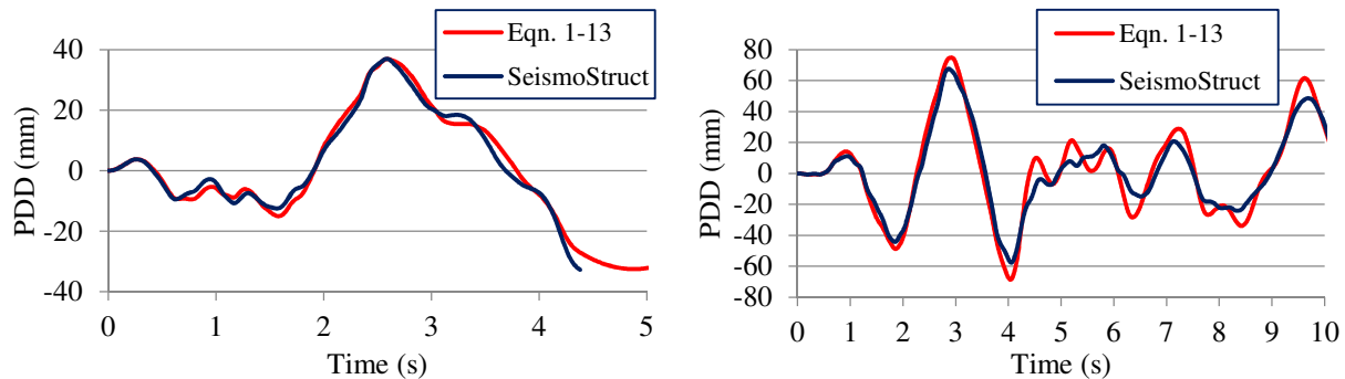
Figure 6. Time-history analysis and SeismoStruct results for (a) building type 1 with soil class B motion and (b) building type 2 with soil class D motion
