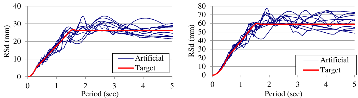
Figure 5. Displacement response of artificial motions for (a) soil class B and (b) soil class D
