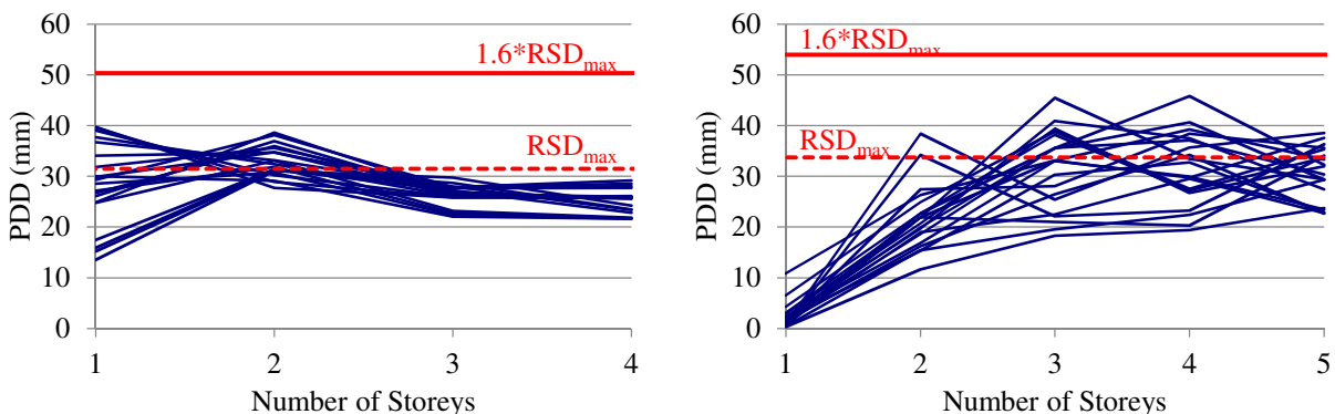
Figure 4. PDD as a function of the number of storeys for different floor areas and for (a) building Type 1 and (b) building Type 2
