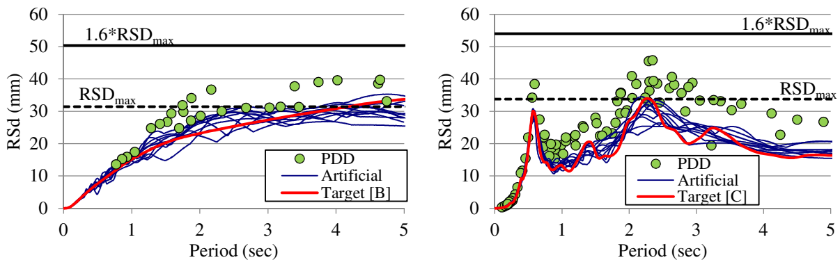
Figure 3. Displacement response of artificial motions for (a) soil class B, building Type 1 and (b) soil class C, building Type 2
